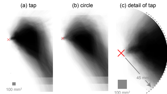
Figure 9. Mean occlusion shapes: (a) tap task; (b) circle task; (c) detail of tapping mean shape.
