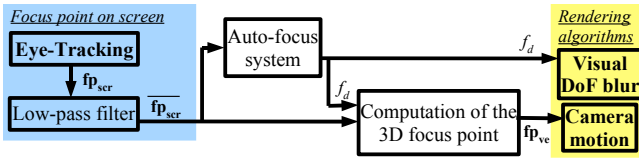
Figure 1: Software architecture.
